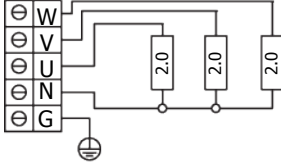
ARI3-60NS-WL 6,0 kW
